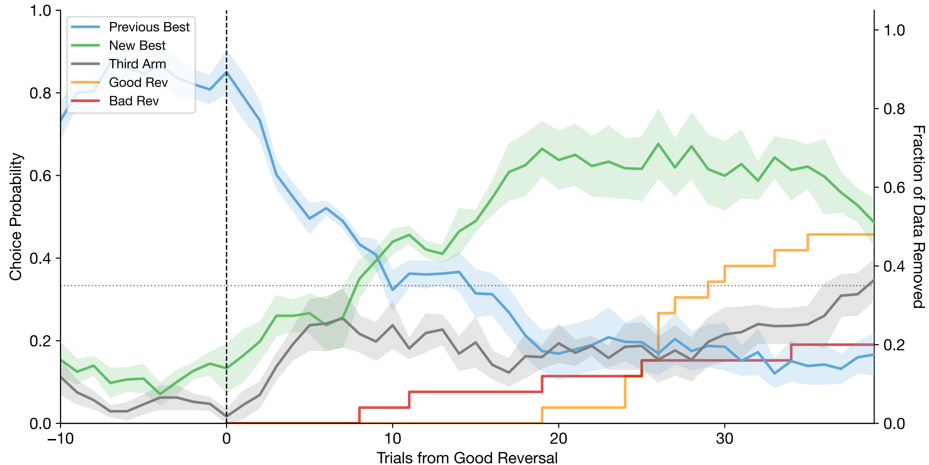
Good Reversal-Aligned Choices (mean \pm se across subjects | n=6 subjects, n=25 reversals)
